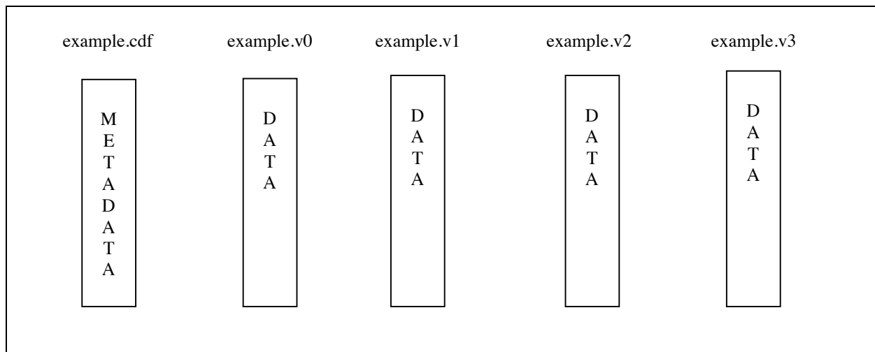
Figure 1.4 Multi-File Format
