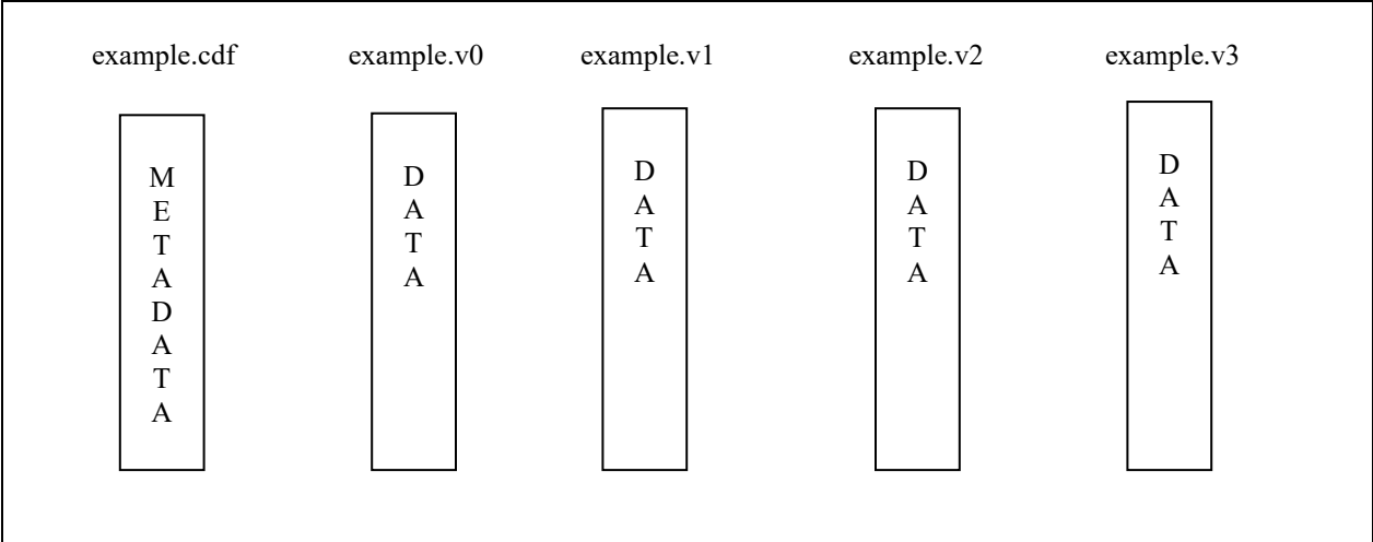
Figure 1.4 Multi-File Format
