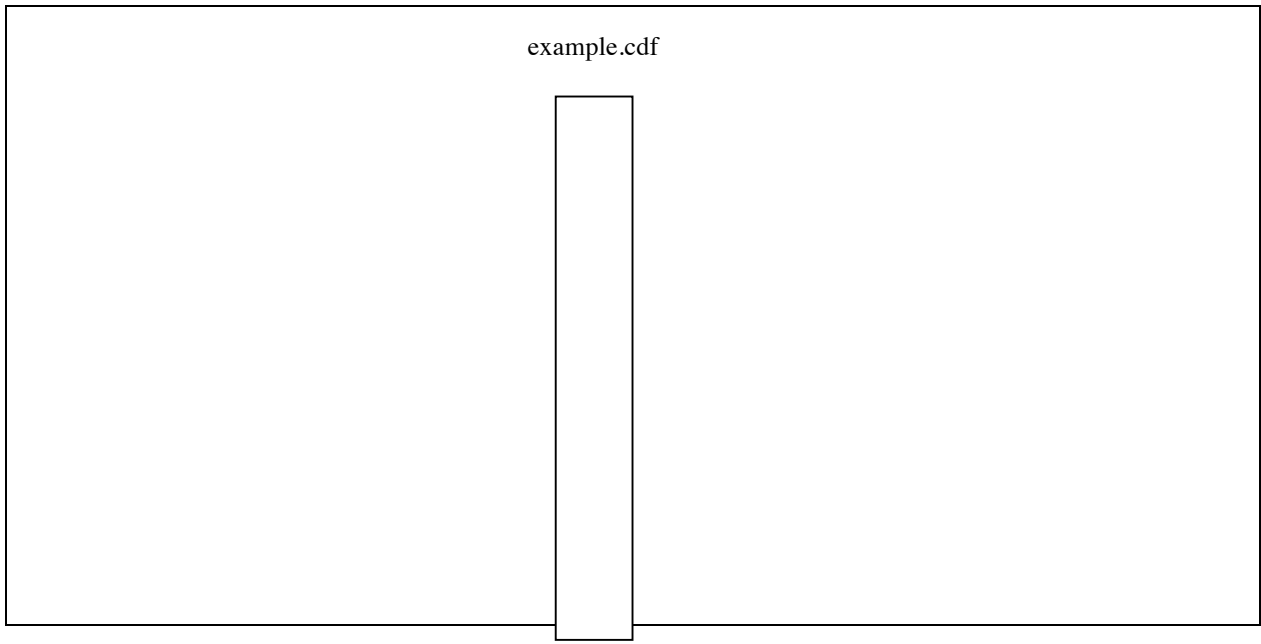
Figure 1.5 Single-File Formats
