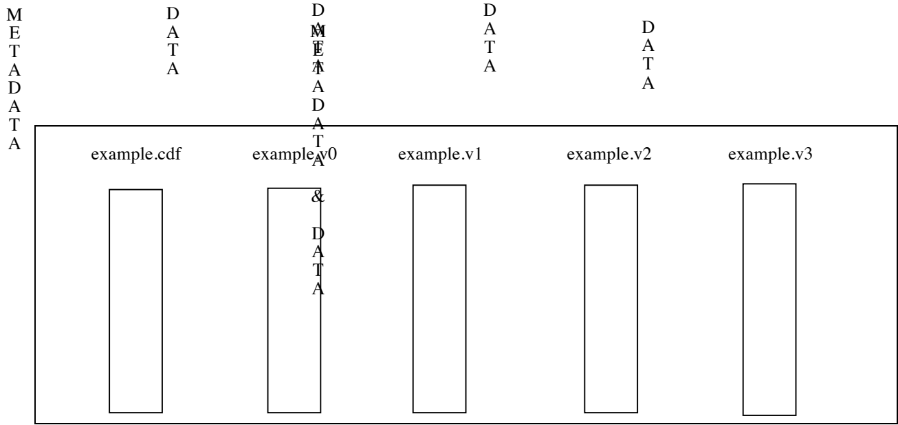
Figure 1.4 Multi-File Format
