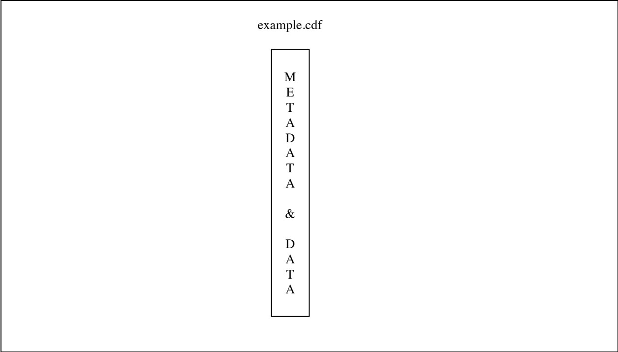
Figure 1.5 Single-File Formats
