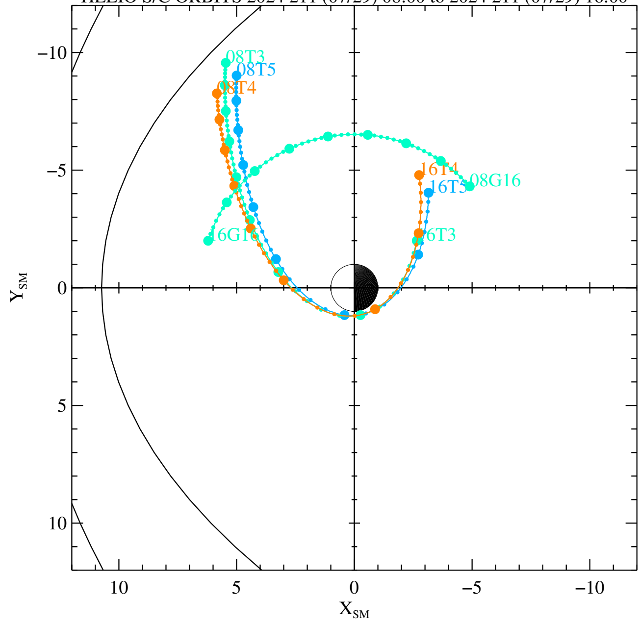
HELIO S/C ORBITS 2024 211 (07/29) 08:00 to 2024 211 (07/29) 16:00
