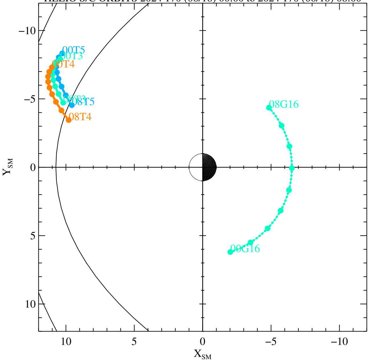
HELIO S/C ORBITS 2024 170 (06/18) 00:00 to 2024 170 (06/18) 08:00
