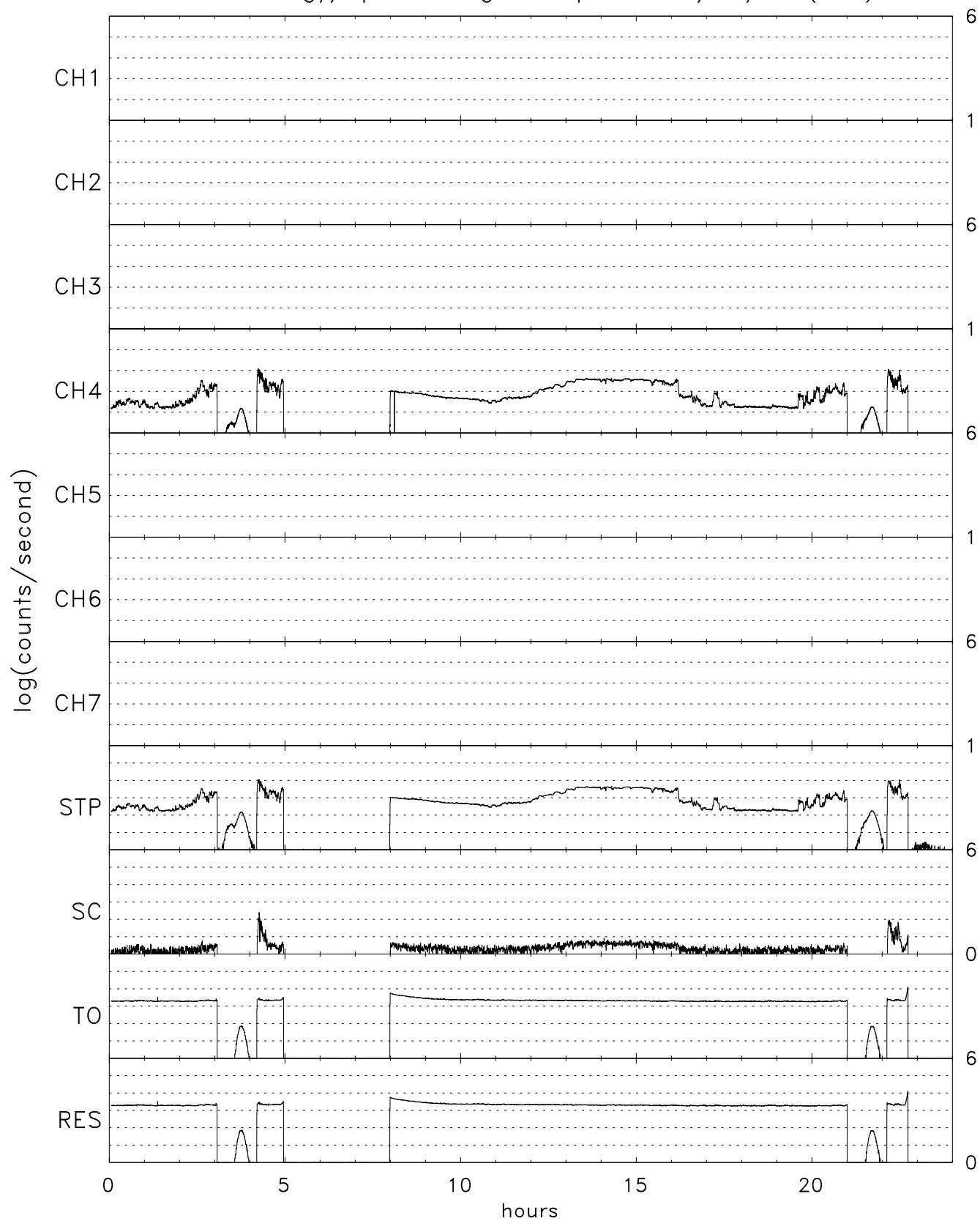
TIDE energy/spin averaged Stops for 12/26/99 (360)
