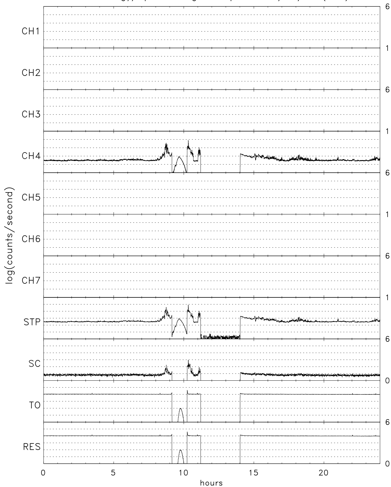
TIDE energy/spin averaged Stops for 11/16/99 (320)
