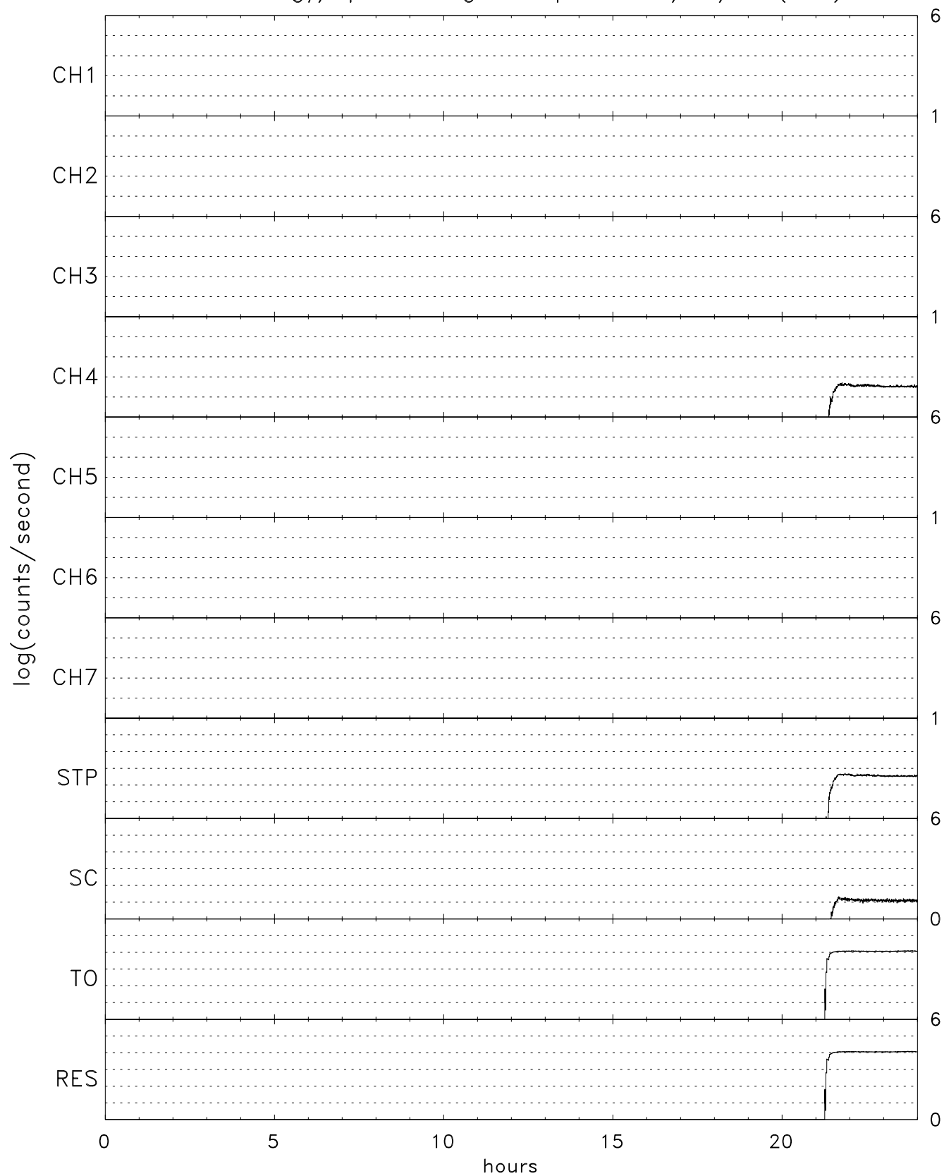
TIDE energy/spin averaged Stops for 10/19/99 (292)
