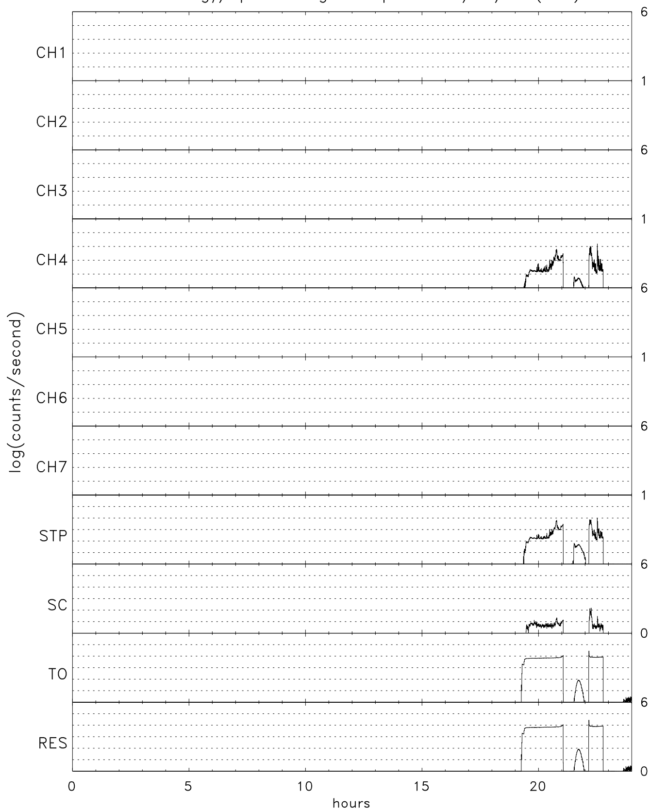
TIDE energy/spin averaged Stops for 10/12/99 (285)
