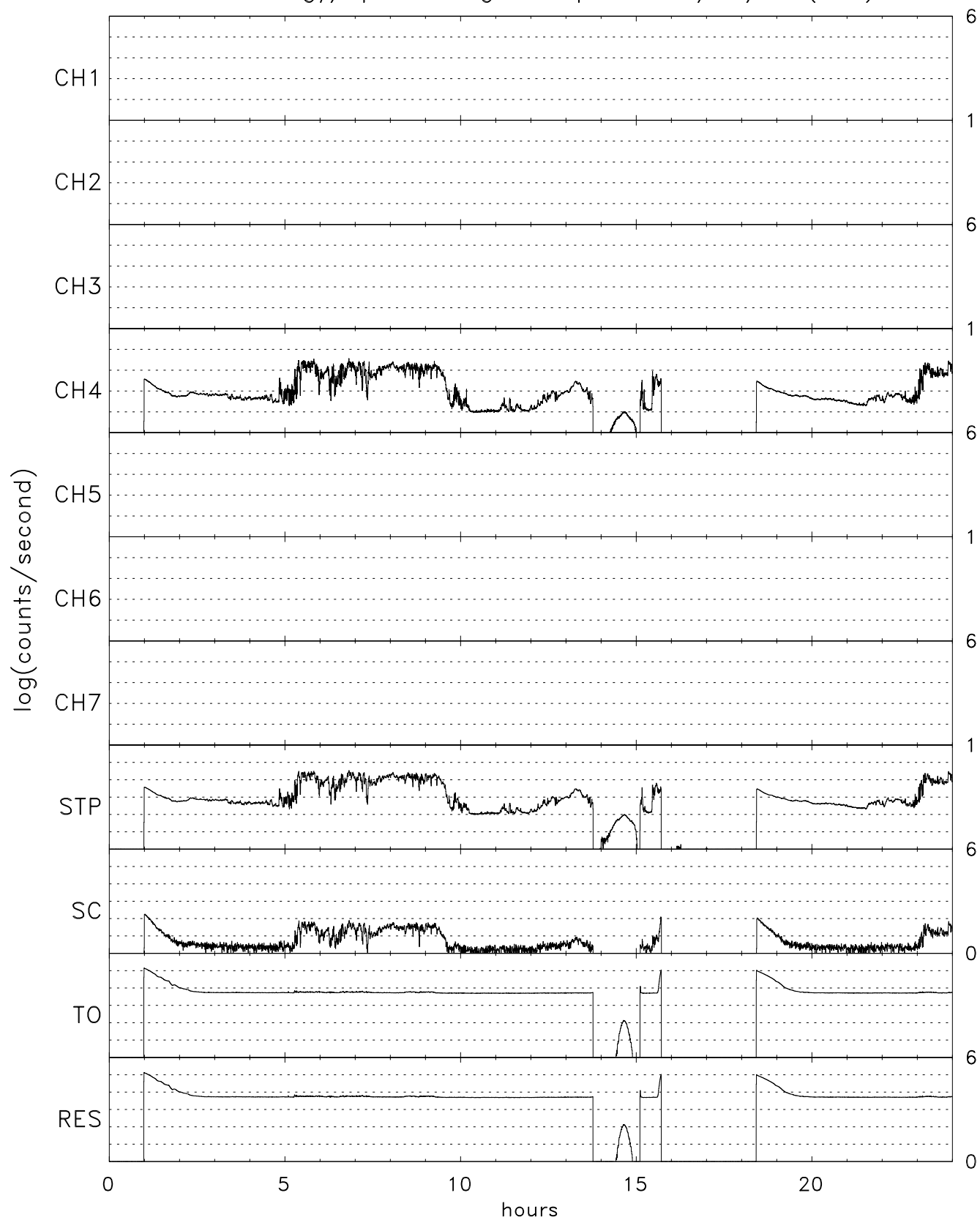
TIDE energy/spin averaged Stops for 05/27/99 (147)
