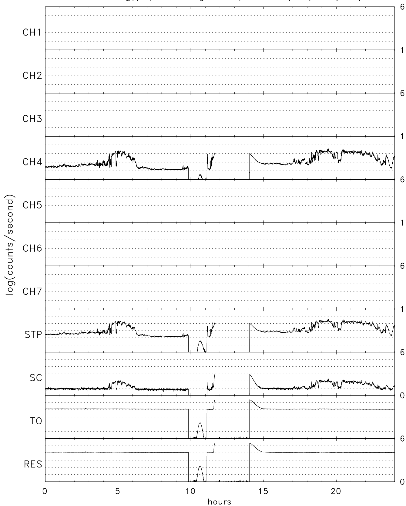
TIDE energy/spin averaged Stops for 05/04/99 (124)
