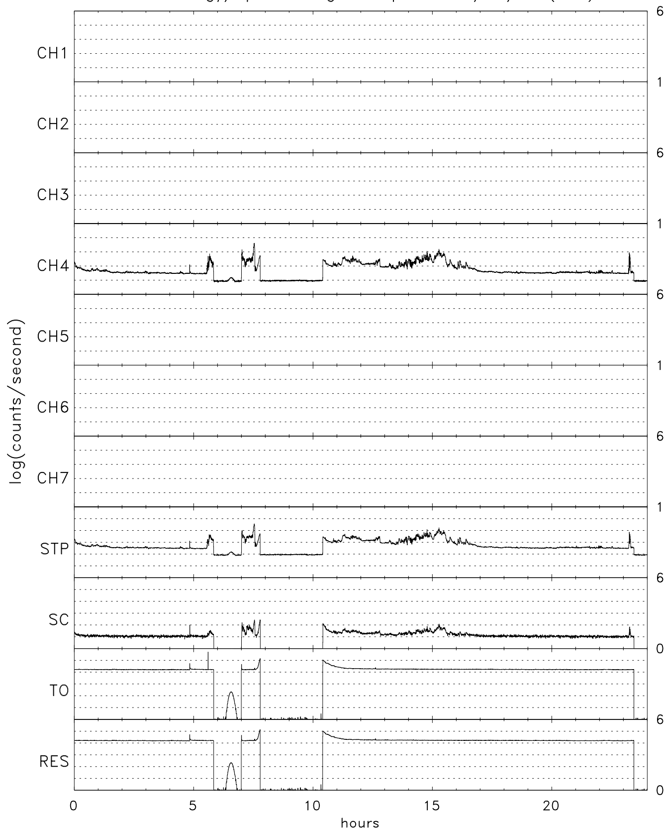
TIDE energy/spin averaged Stops for 03/07/99 (066)
