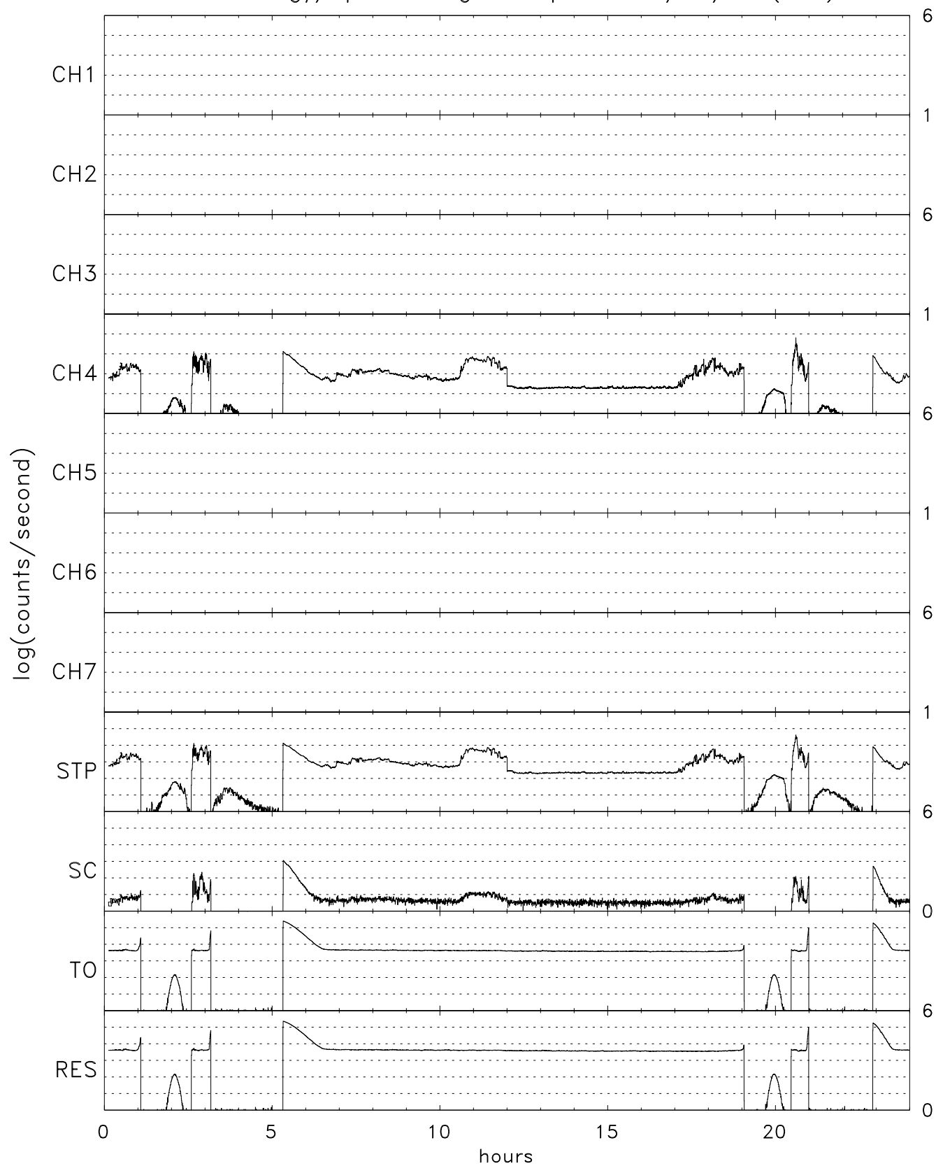
TIDE energy/spin averaged Stops for 12/22/98 (356)
