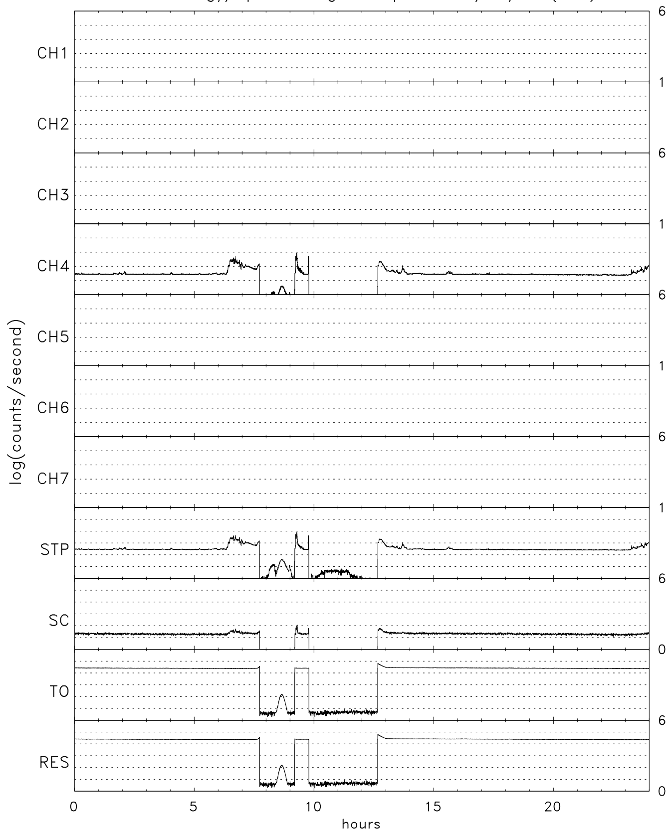
TIDE energy/spin averaged Stops for 11/16/98 (320)
