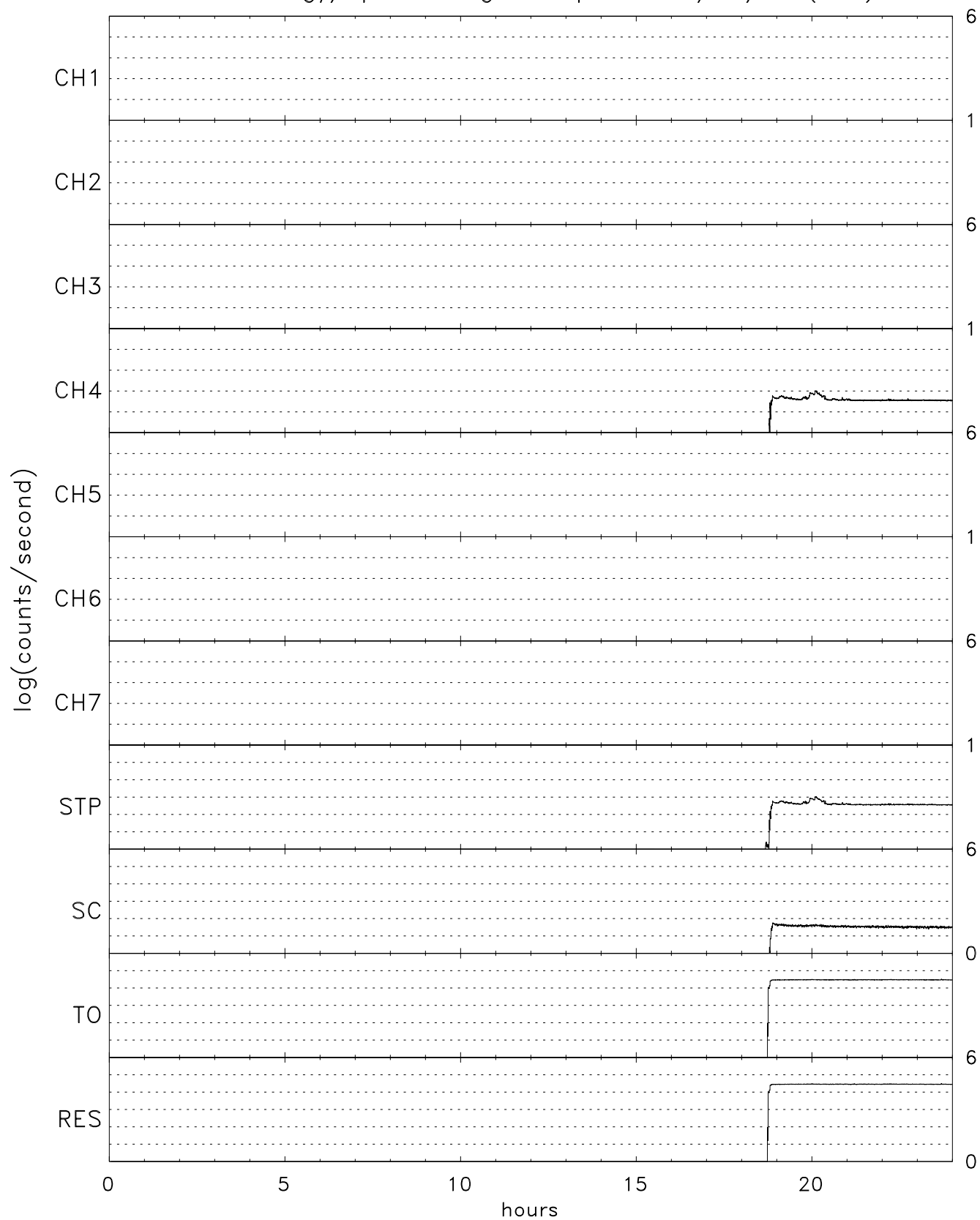
TIDE energy/spin averaged Stops for 10/26/98 (299)
