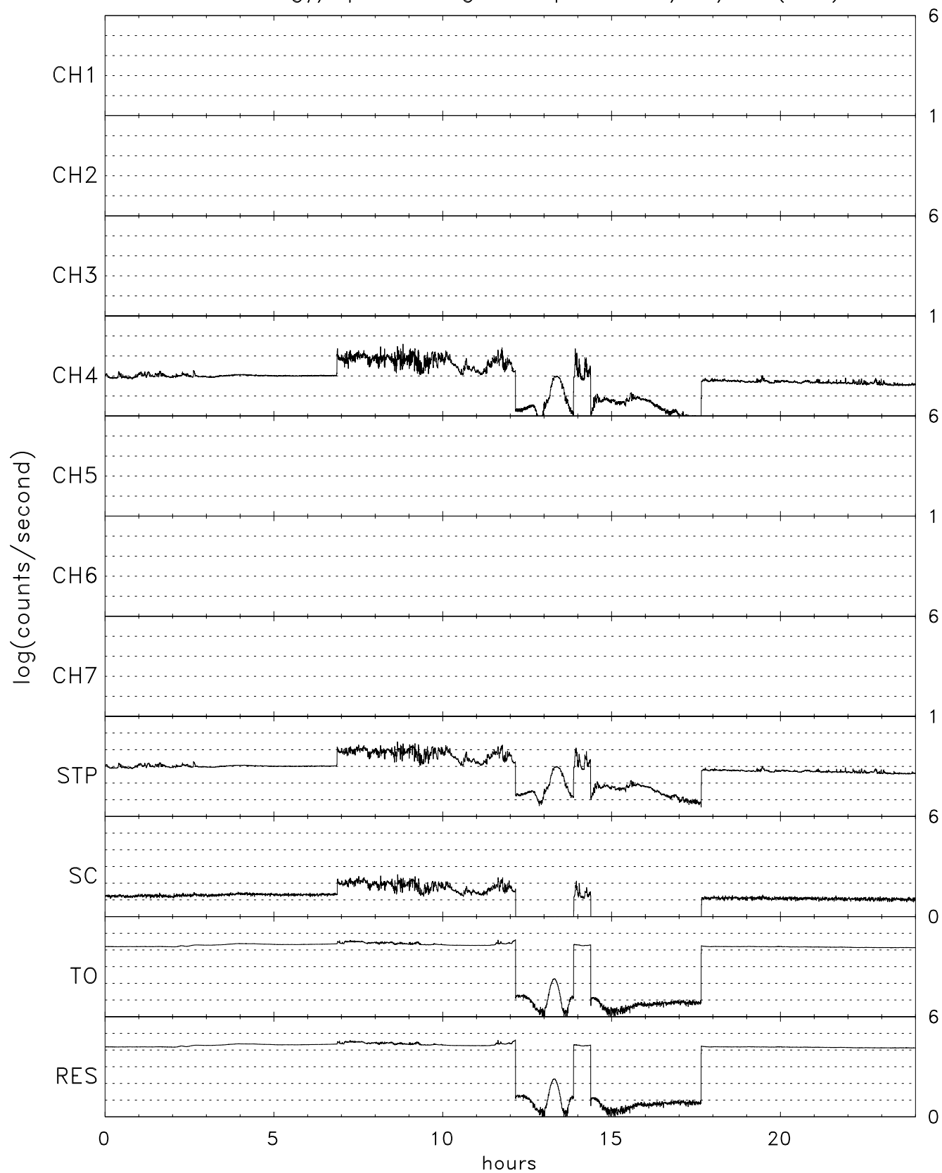
TIDE energy/spin averaged Stops for 08/26/98 (238)
