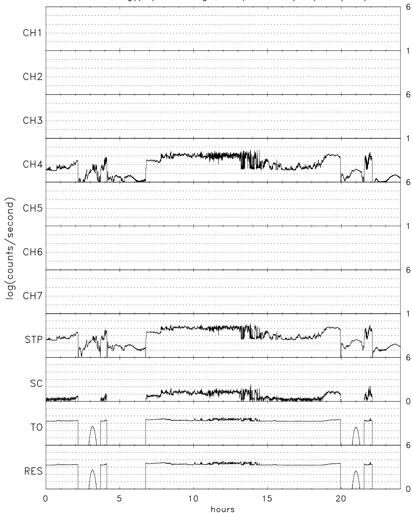
TIDE energy/spin averaged Stops for 06/25/98 (176)
