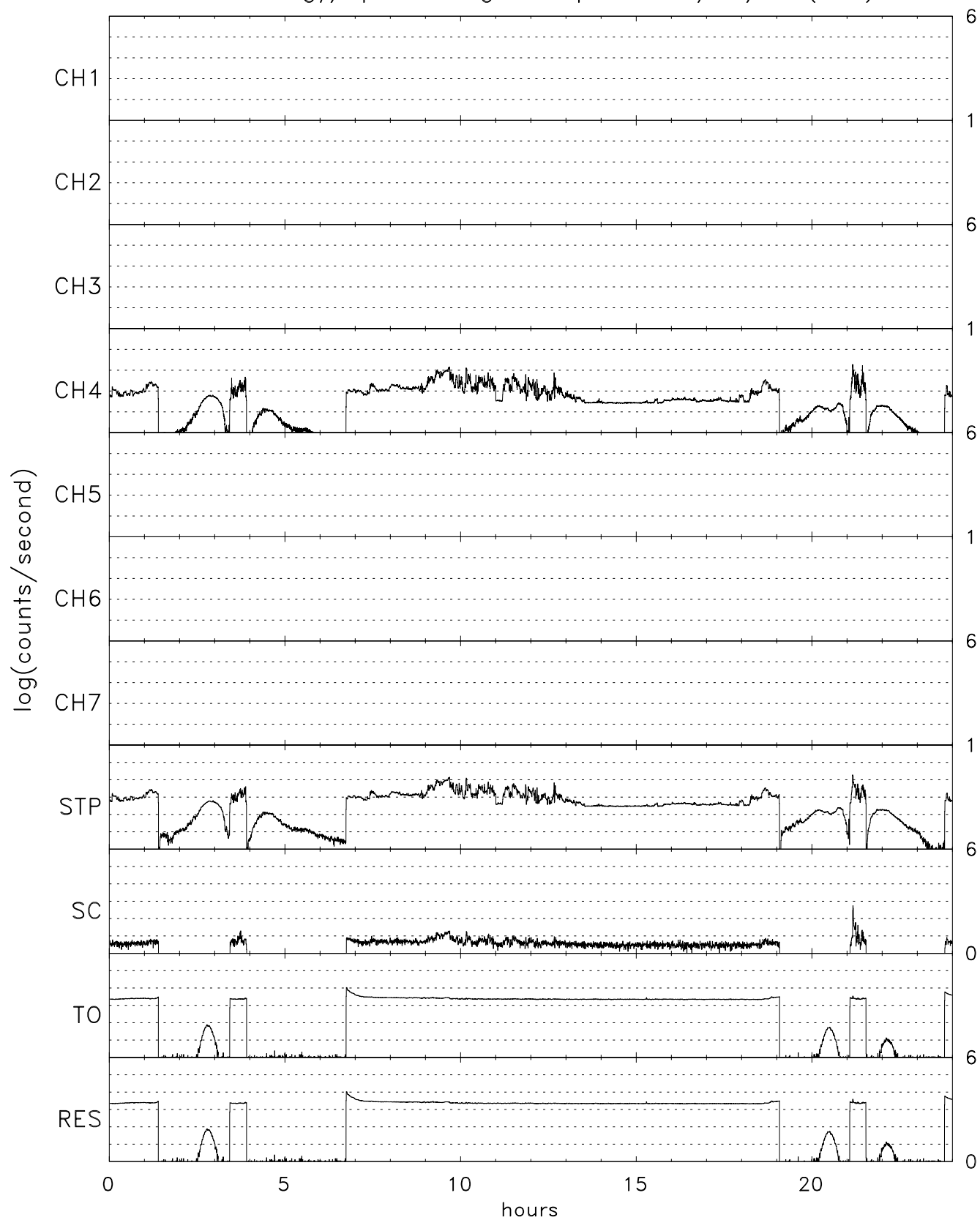
TIDE energy/spin averaged Stops for 01/24/98 (024)
