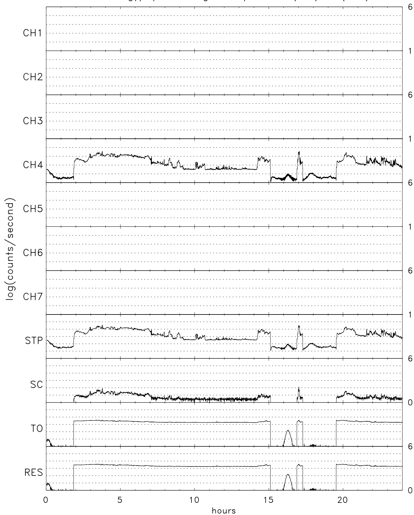
TIDE energy/spin averaged Stops for 01/19/98 (019)
