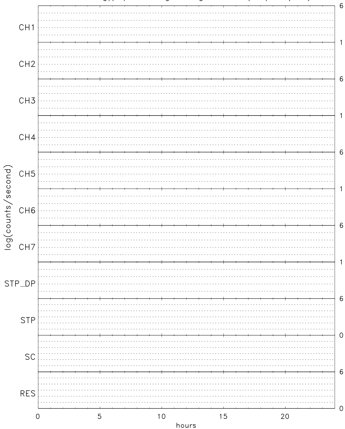
TIDE energy/spin averaged Singles for 11/23/97 (327)
