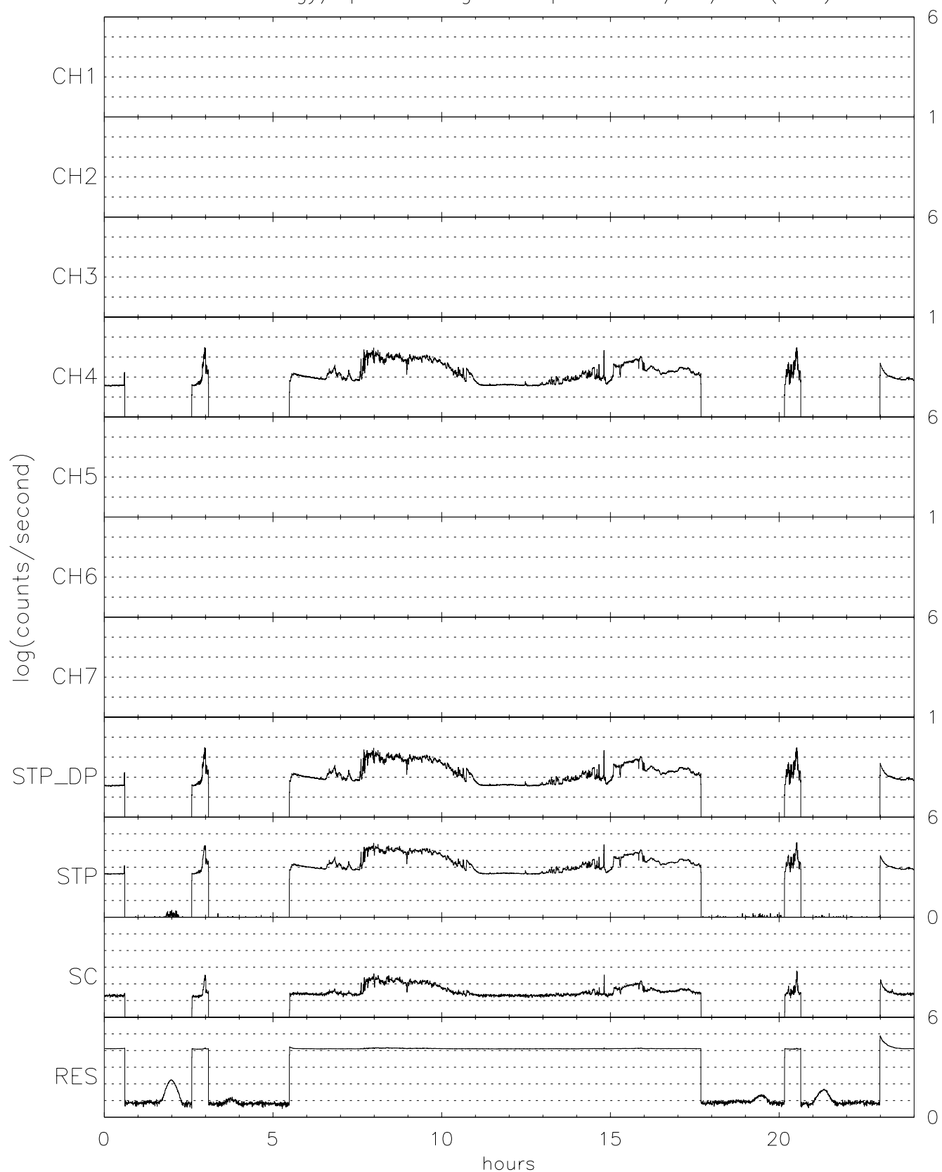
TIDE energy/spin averaged Stops for 05/07/97 (127)
