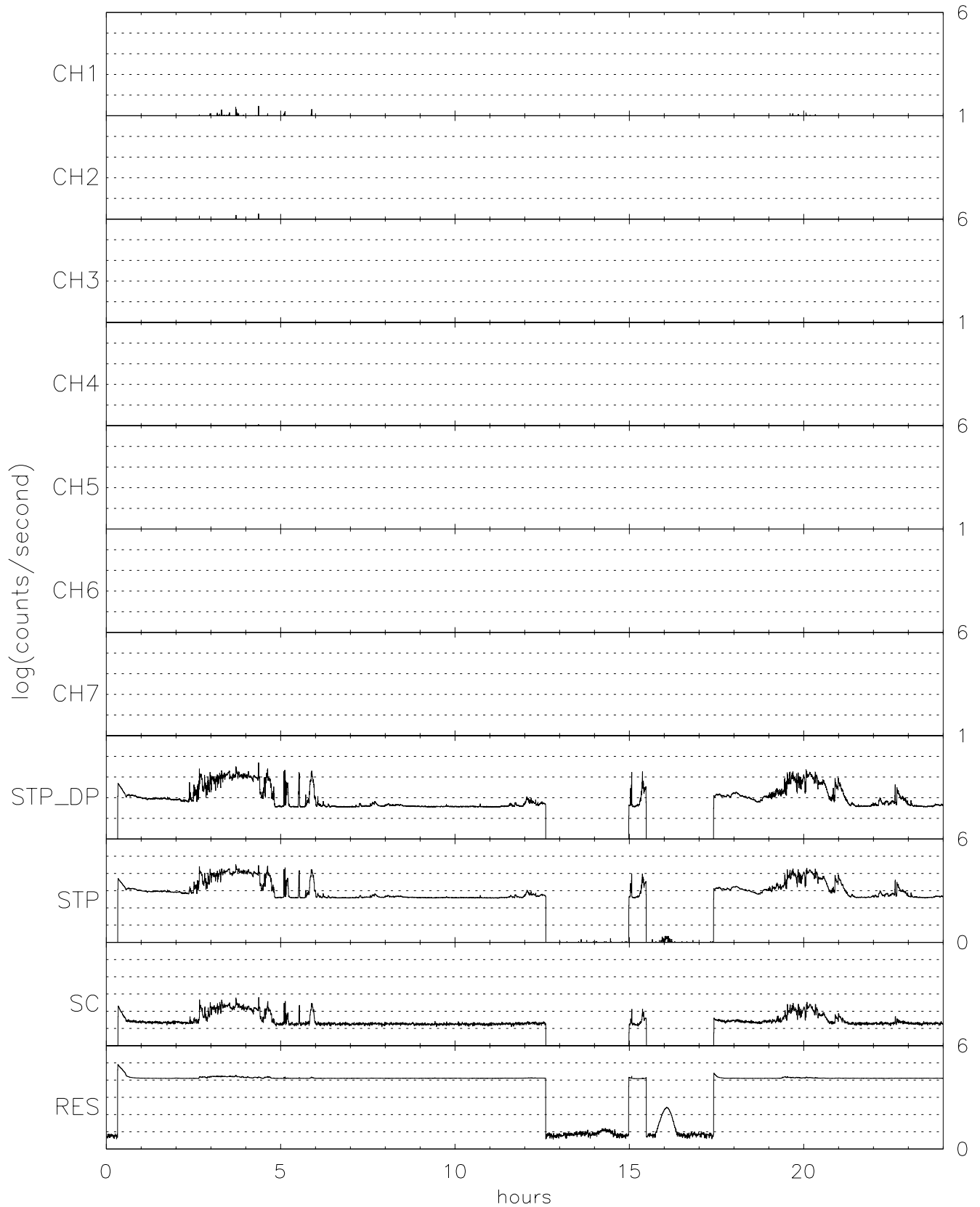
TIDE energy/spin averaged H+ for 05/05/97 (125)
