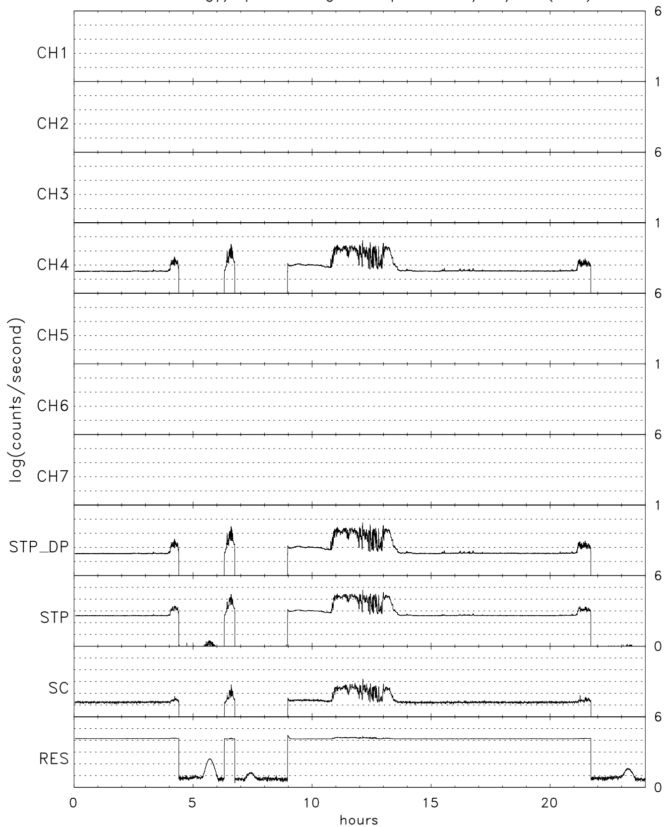
TIDE energy/spin averaged Stops for 04/28/97 (118)
