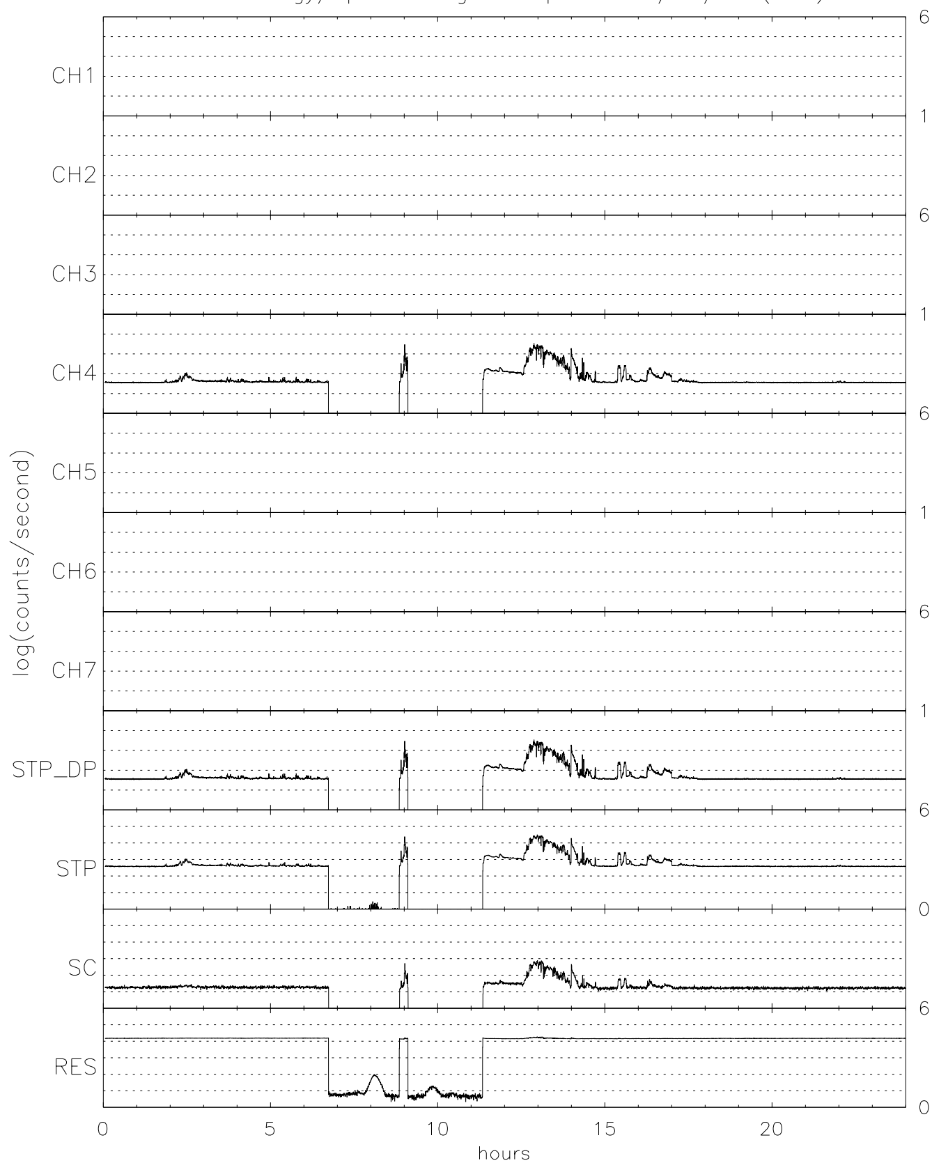
TIDE energy/spin averaged Stops for 04/22/97 (112)
