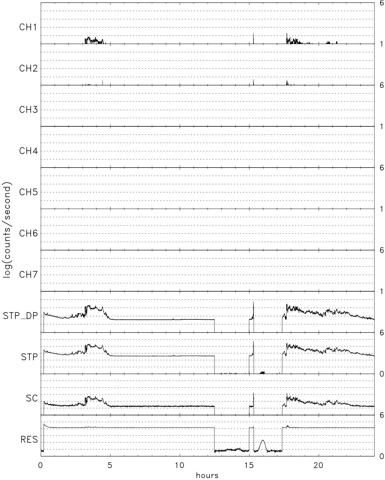
TIDE energy/spin averaged H+ for 04/21/97 (111)
