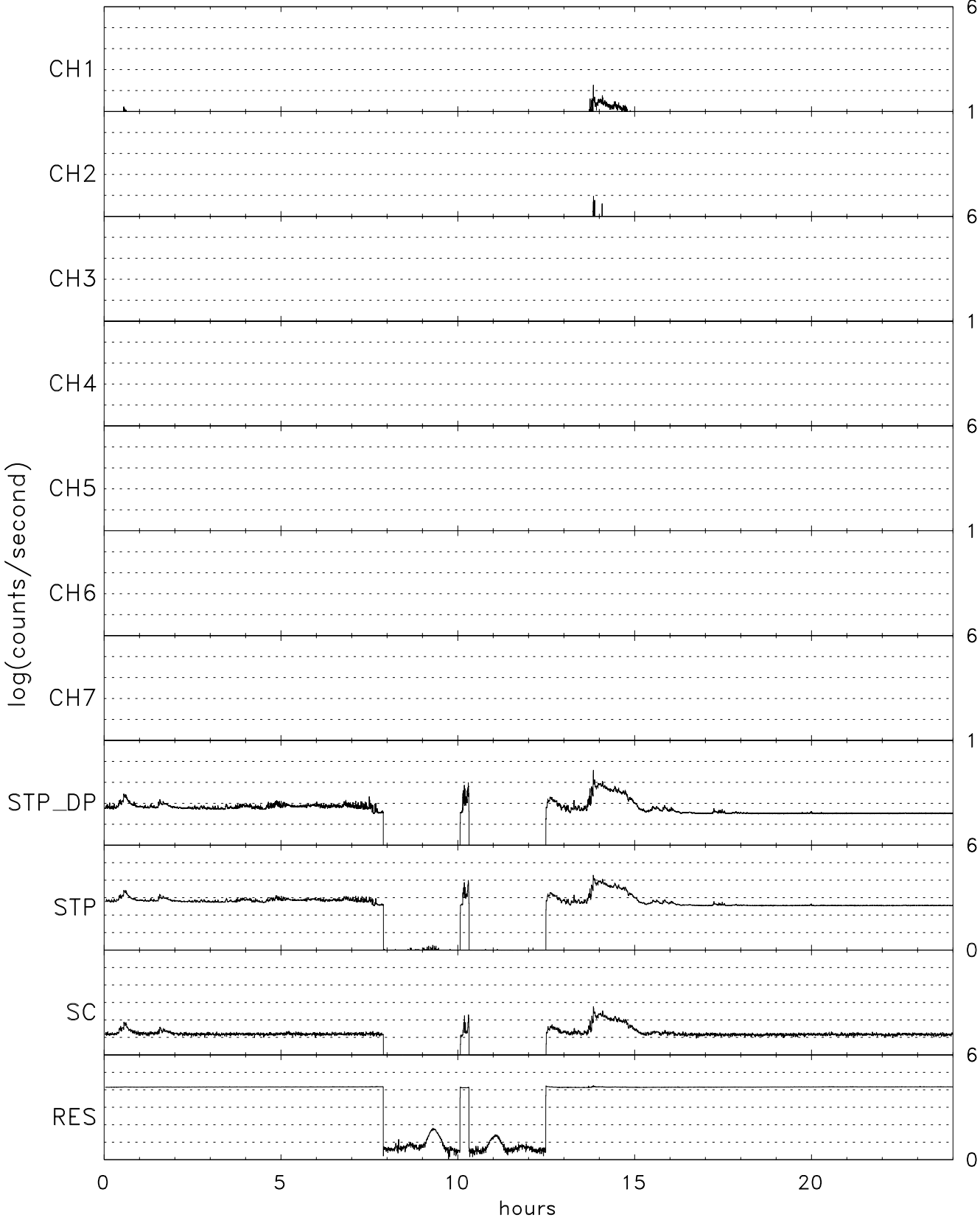
TIDE energy/spin averaged H+ for 04/19/97 (109)
