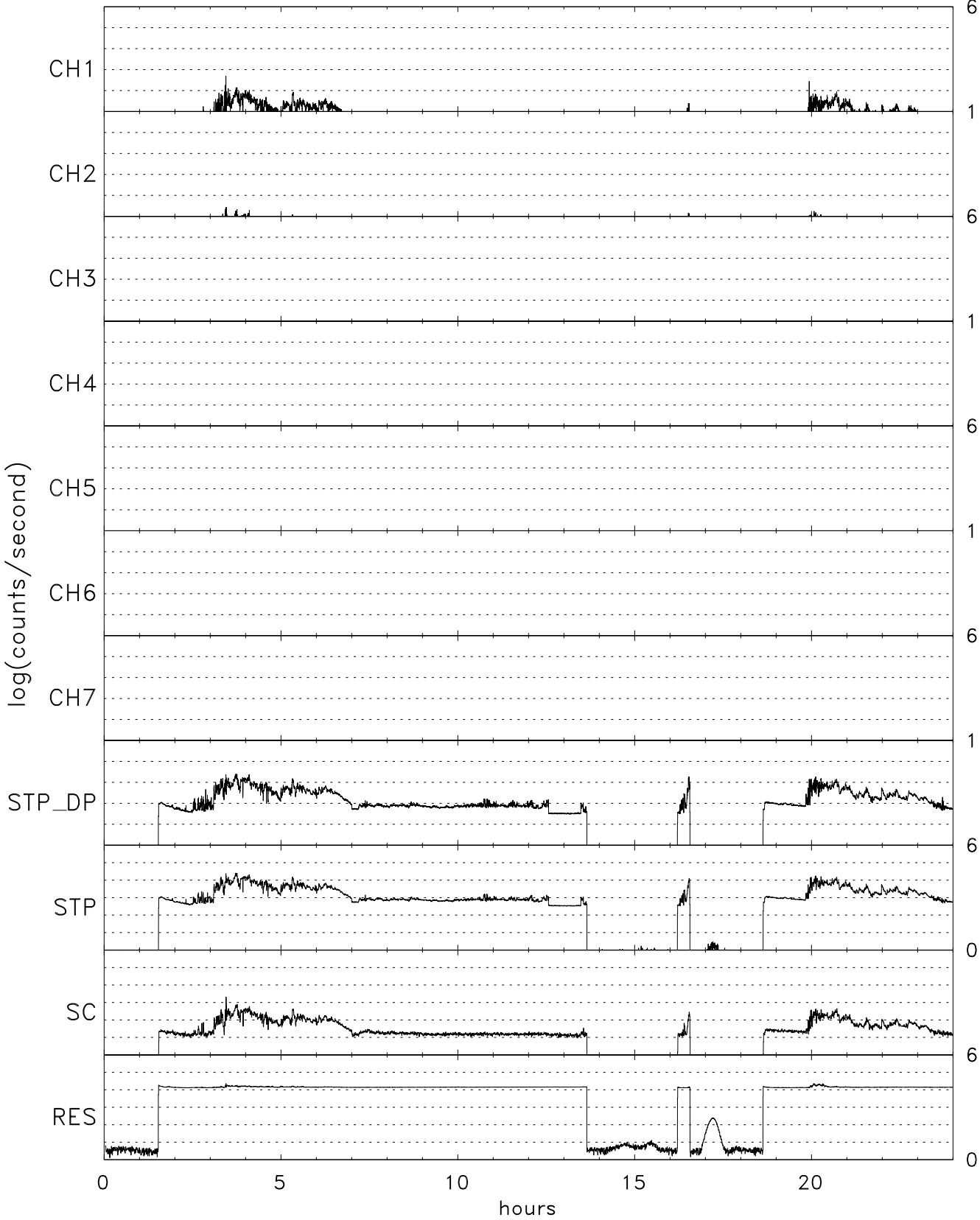
TIDE energy/spin averaged H+ for 04/18/97 (108)
