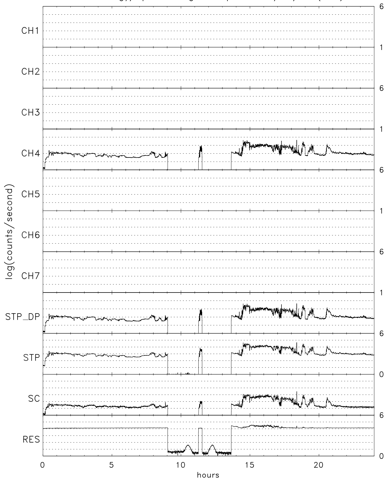
TIDE energy/spin averaged Stops for 04/16/97 (106)
