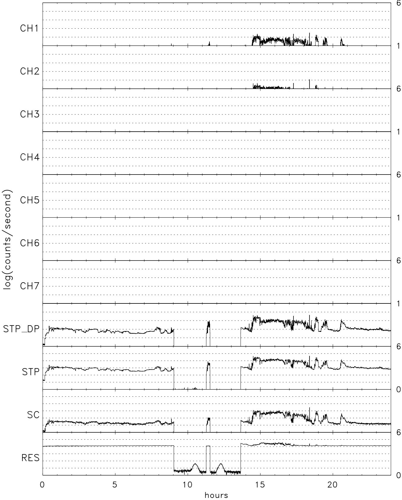
TIDE energy/spin averaged H+ for 04/16/97 (106)
