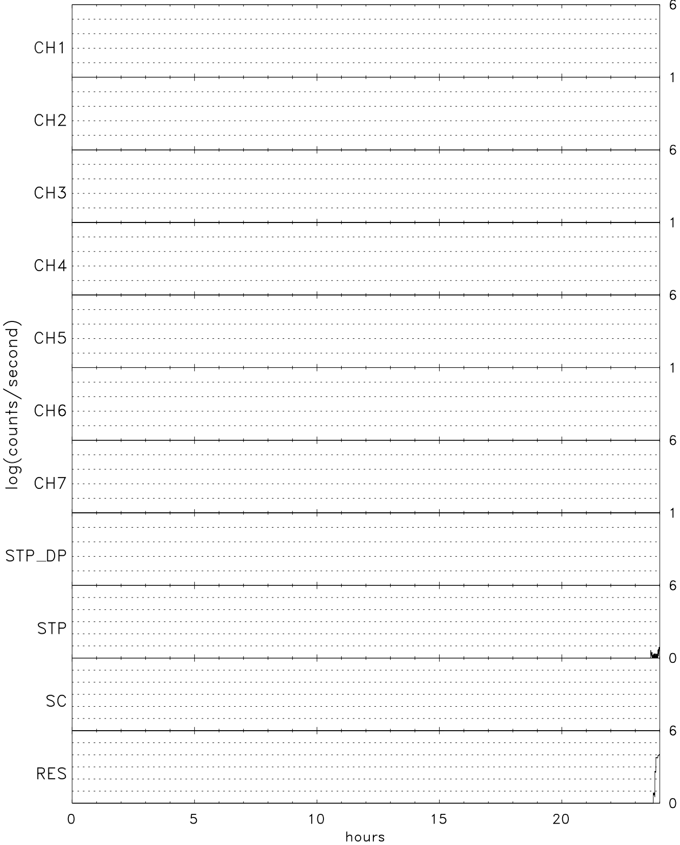
TIDE energy/spin averaged H+ for 04/15/97 (105)
