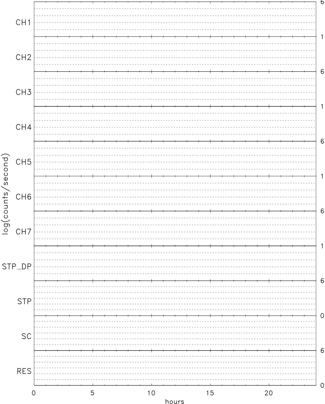
TIDE energy/spin averaged H+ for 04/14/97 (104)
