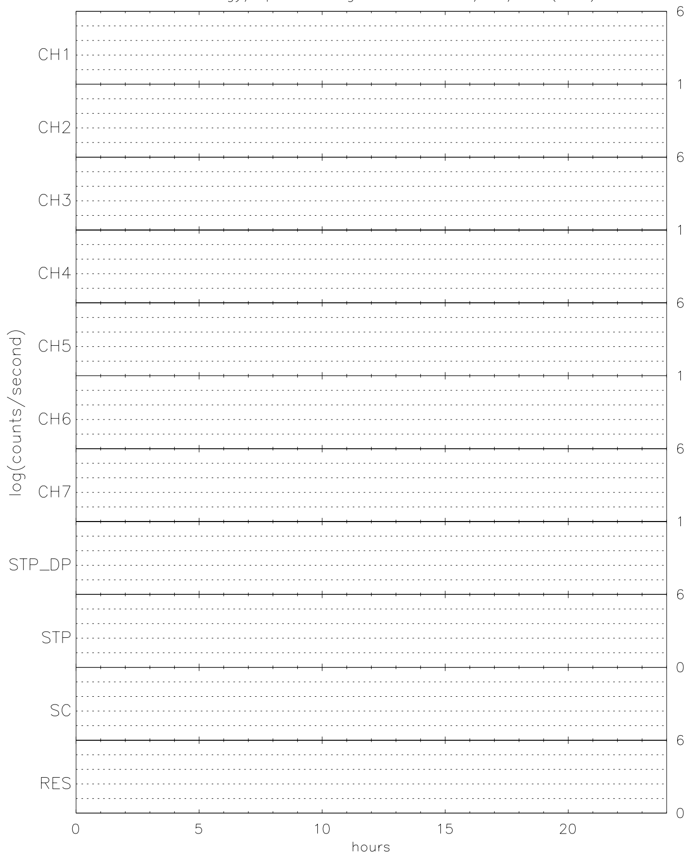
TIDE energy/spin averaged H+ for 04/12/97 (102)
