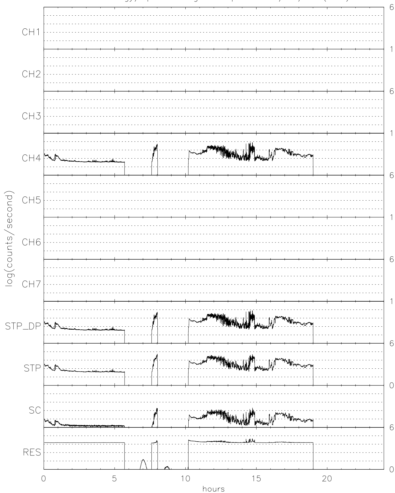
TIDE energy/spin averaged Stops for 04/11/97 (101)
