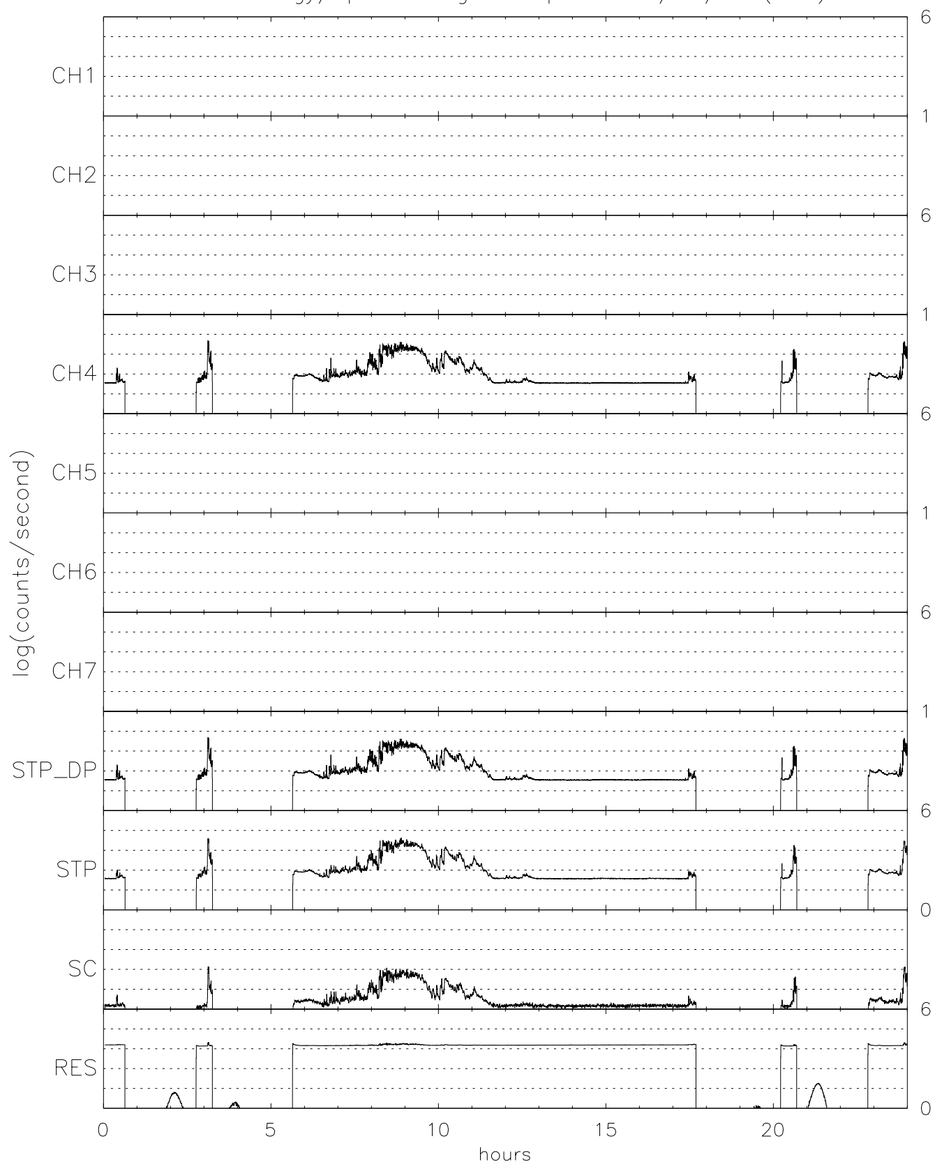
TIDE energy/spin averaged Stops for 04/09/97 (099)
