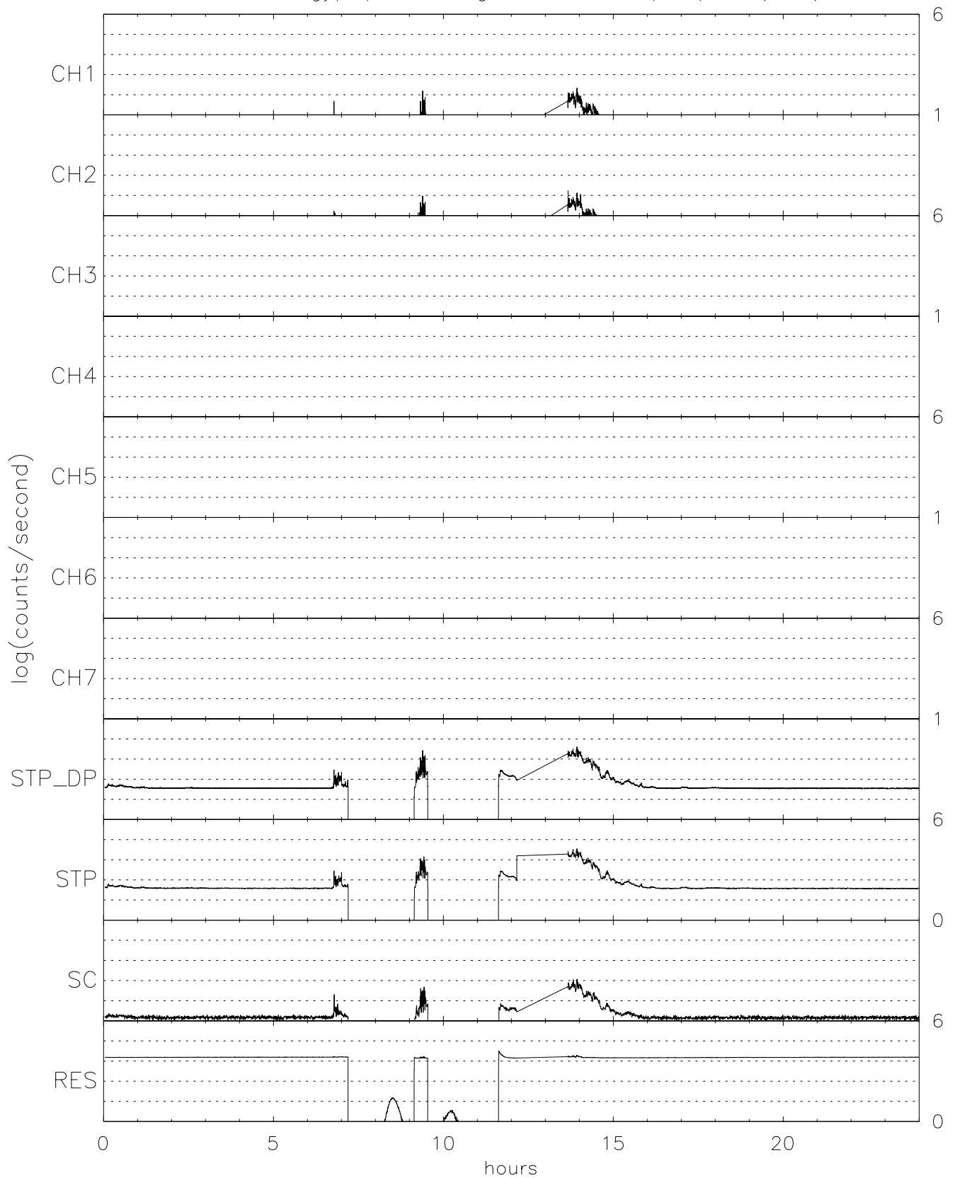
TIDE energy/spin averaged H+ for 04/08/97 (098)
