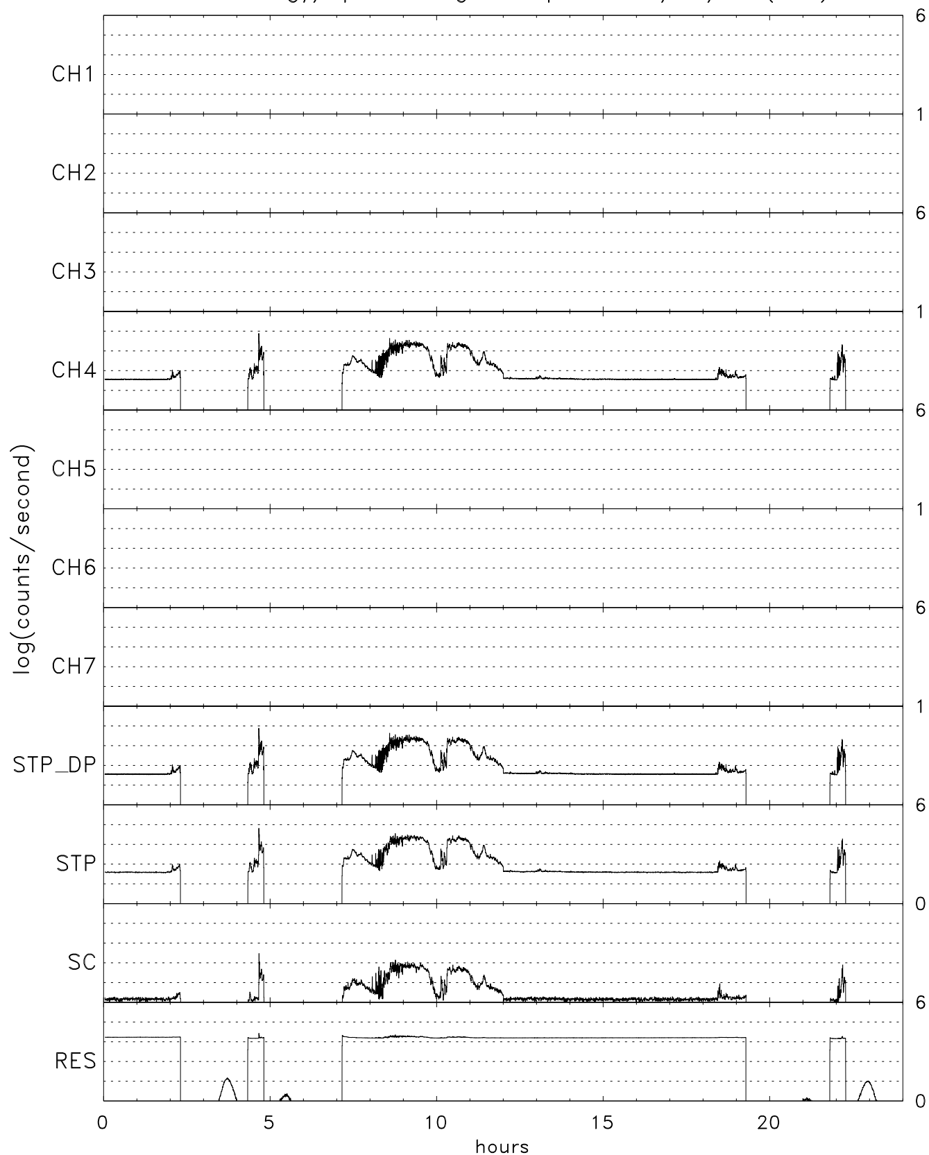
TIDE energy/spin averaged Stops for 04/06/97 (096)
