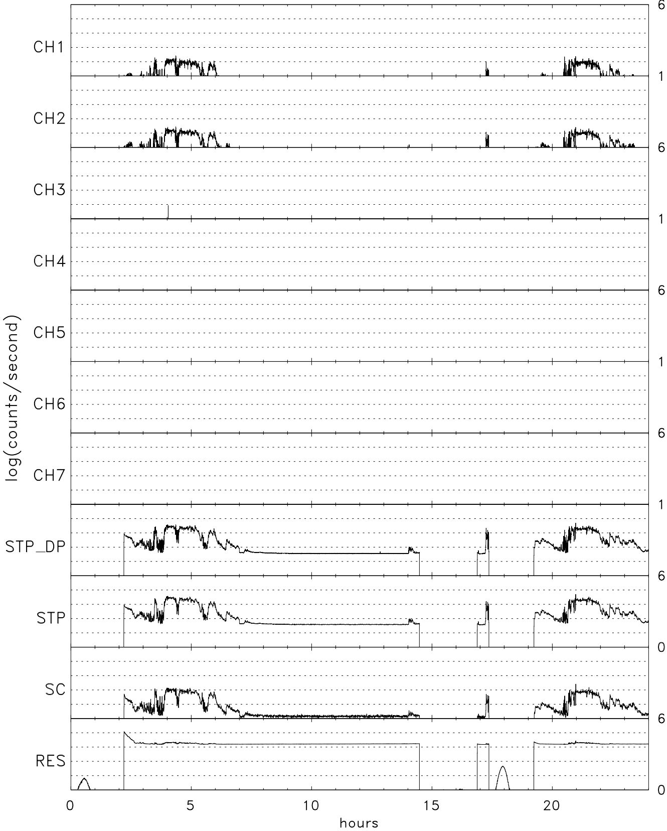
TIDE energy/spin averaged H+ for 04/04/97 (094)
