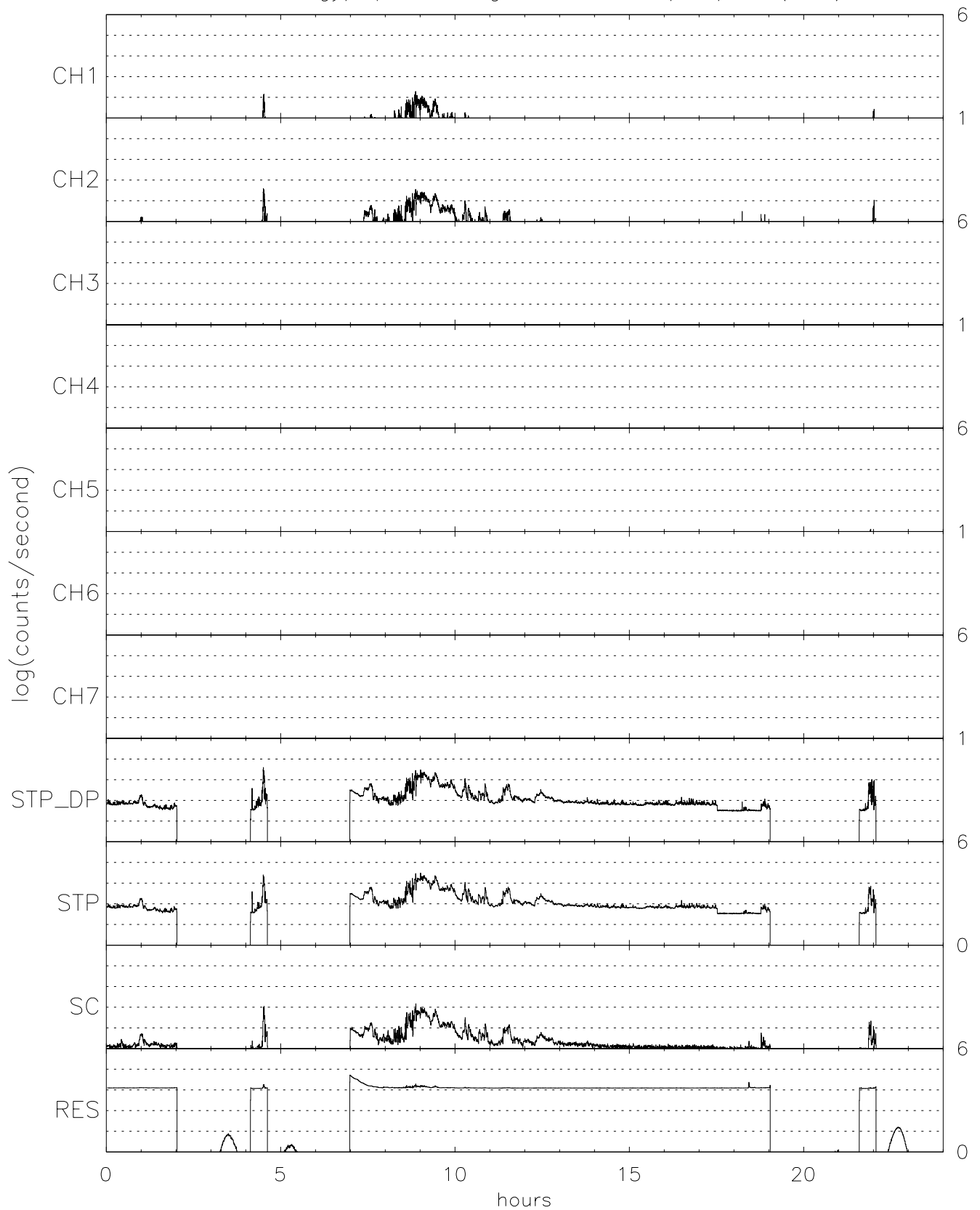
TIDE energy/spin averaged H+ for 03/26/97 (085)
