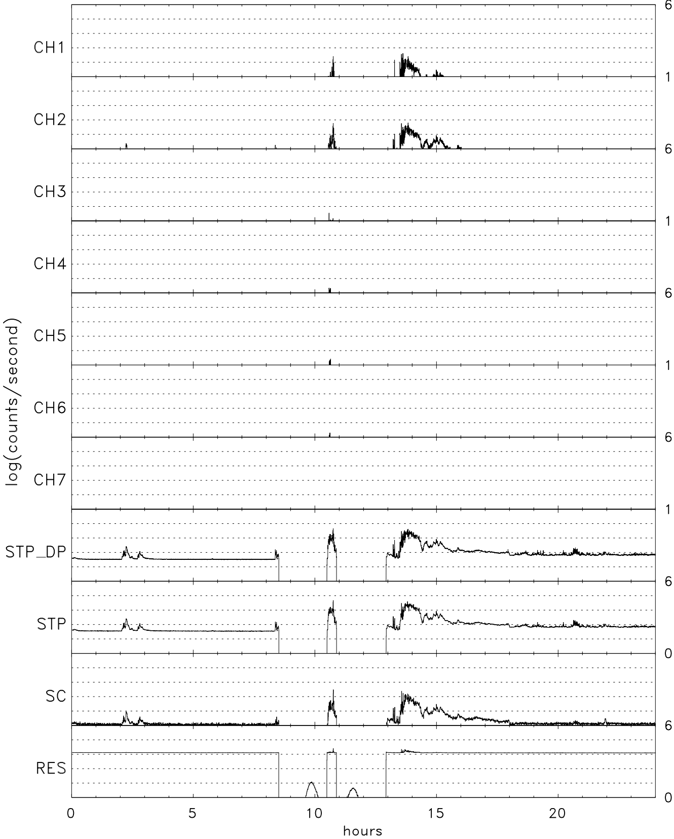
TIDE energy/spin averaged H+ for 03/25/97 (084)
