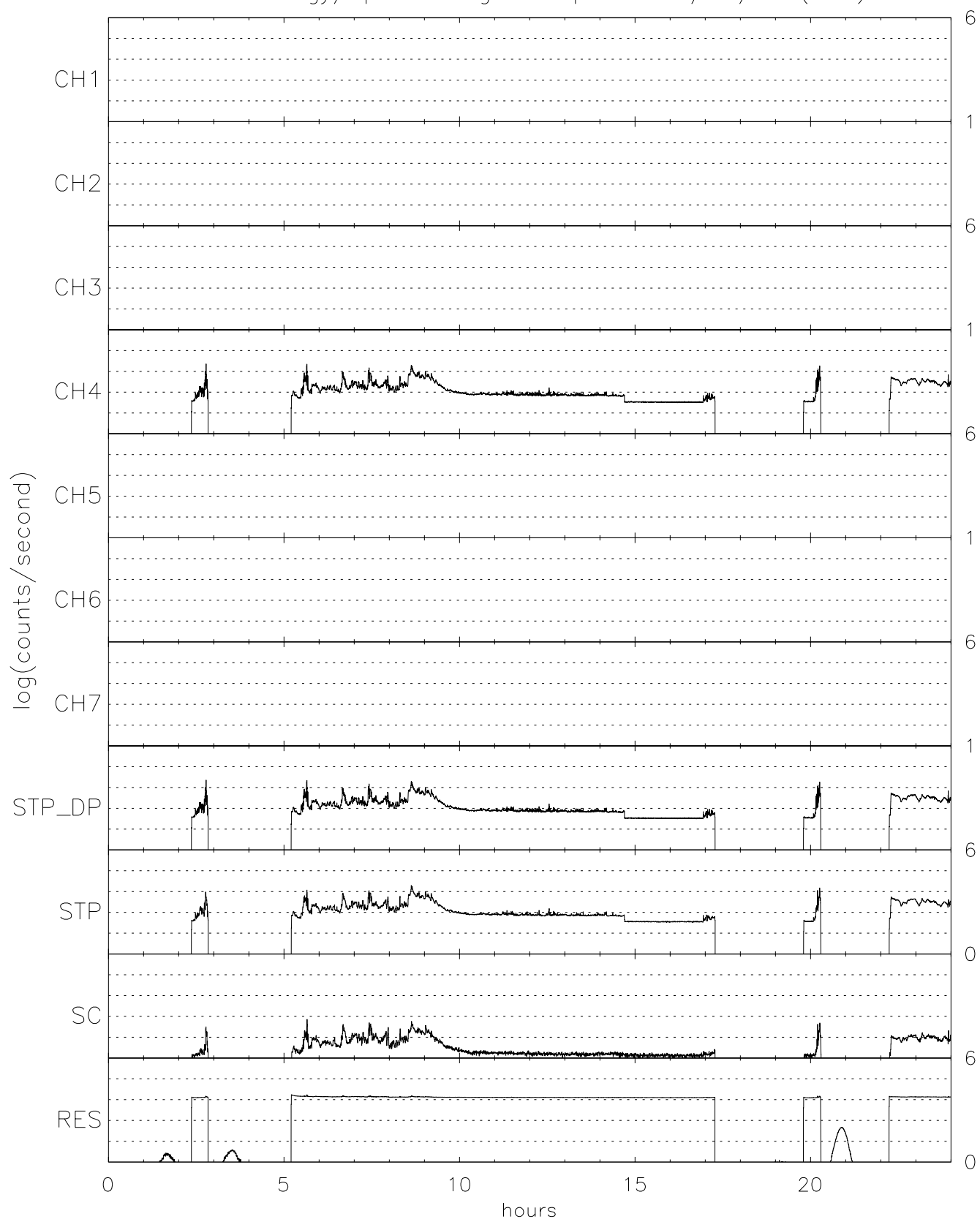
TIDE energy/spin averaged Stops for 03/18/97 (077)
