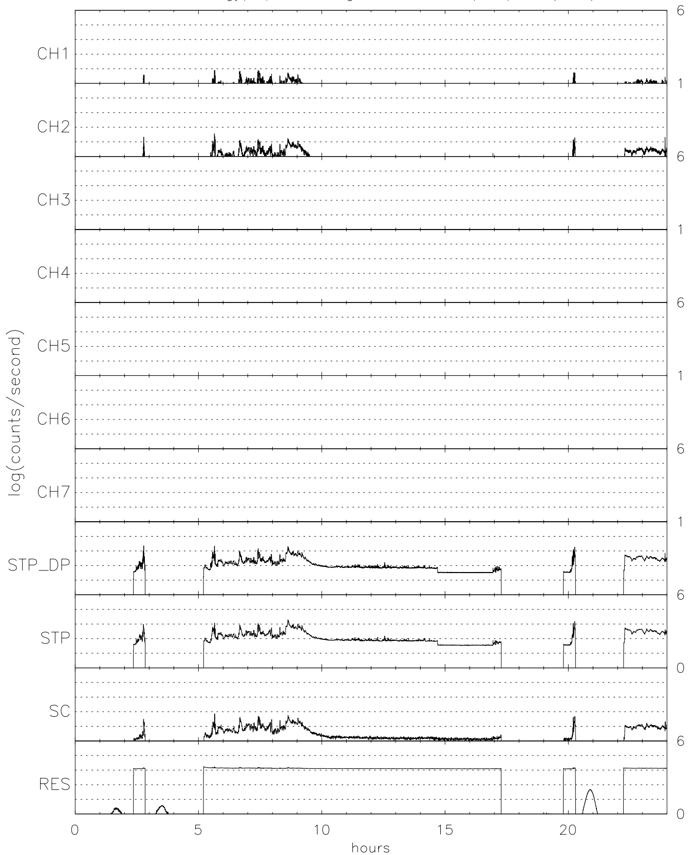
TIDE energy/spin averaged H+ for 03/18/97 (077)
