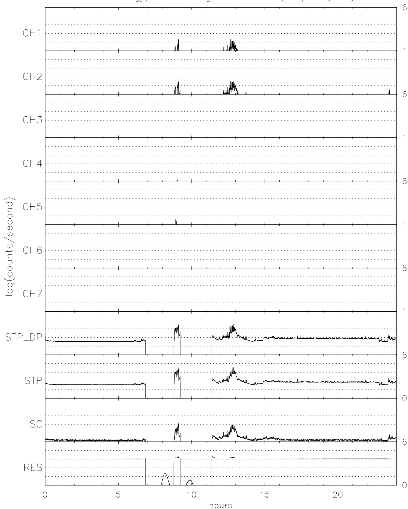
TIDE energy/spin averaged H+ for 03/17/97 (076)
