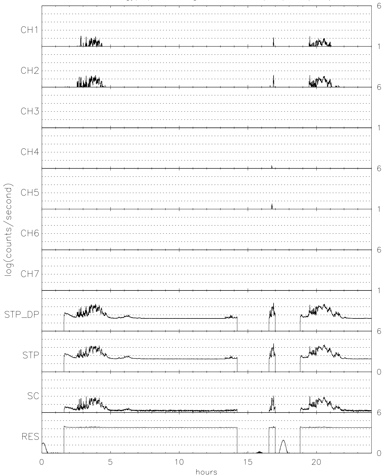
TIDE energy/spin averaged H+ for 03/13/97 (072)
