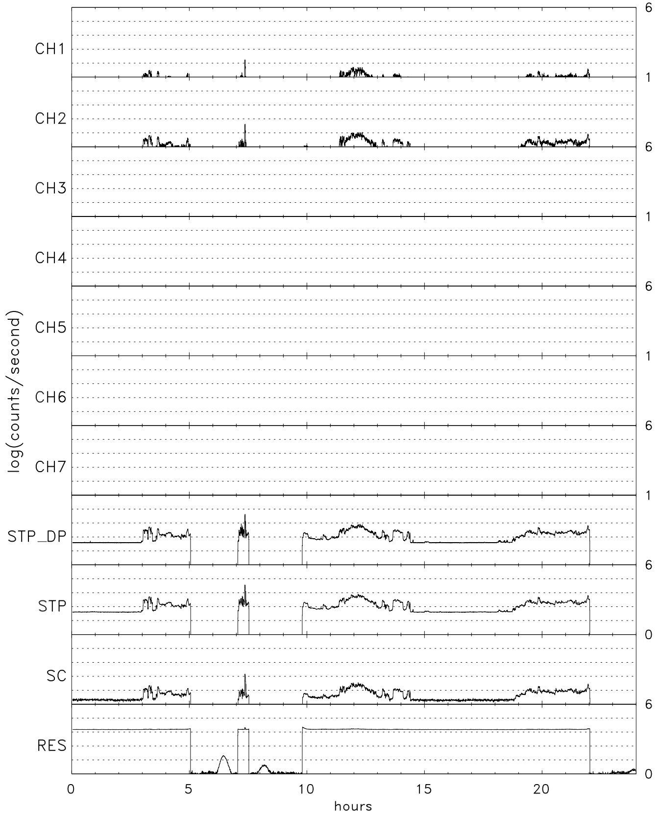
TIDE energy/spin averaged H+ for 03/09/97 (068)
