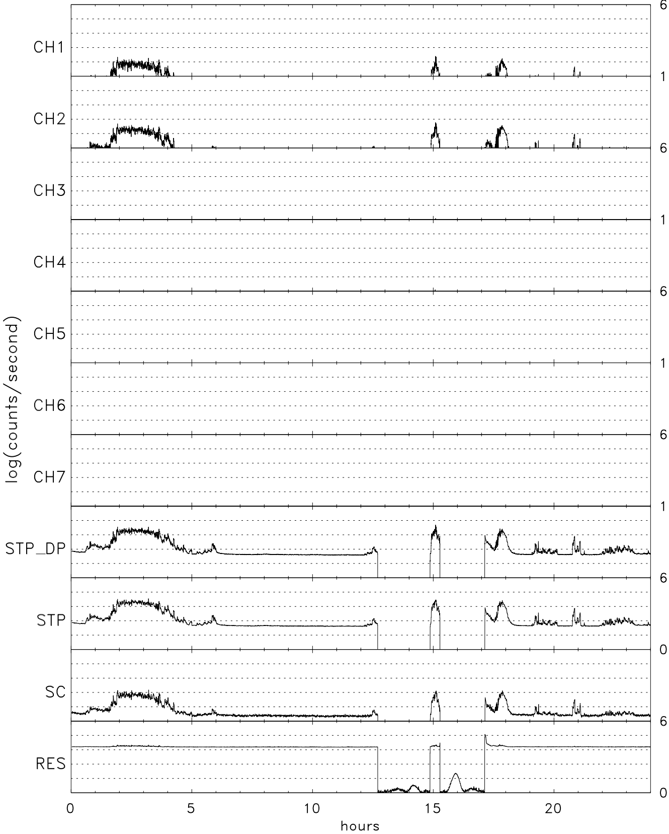
TIDE energy/spin averaged H+ for 03/05/97 (064)
