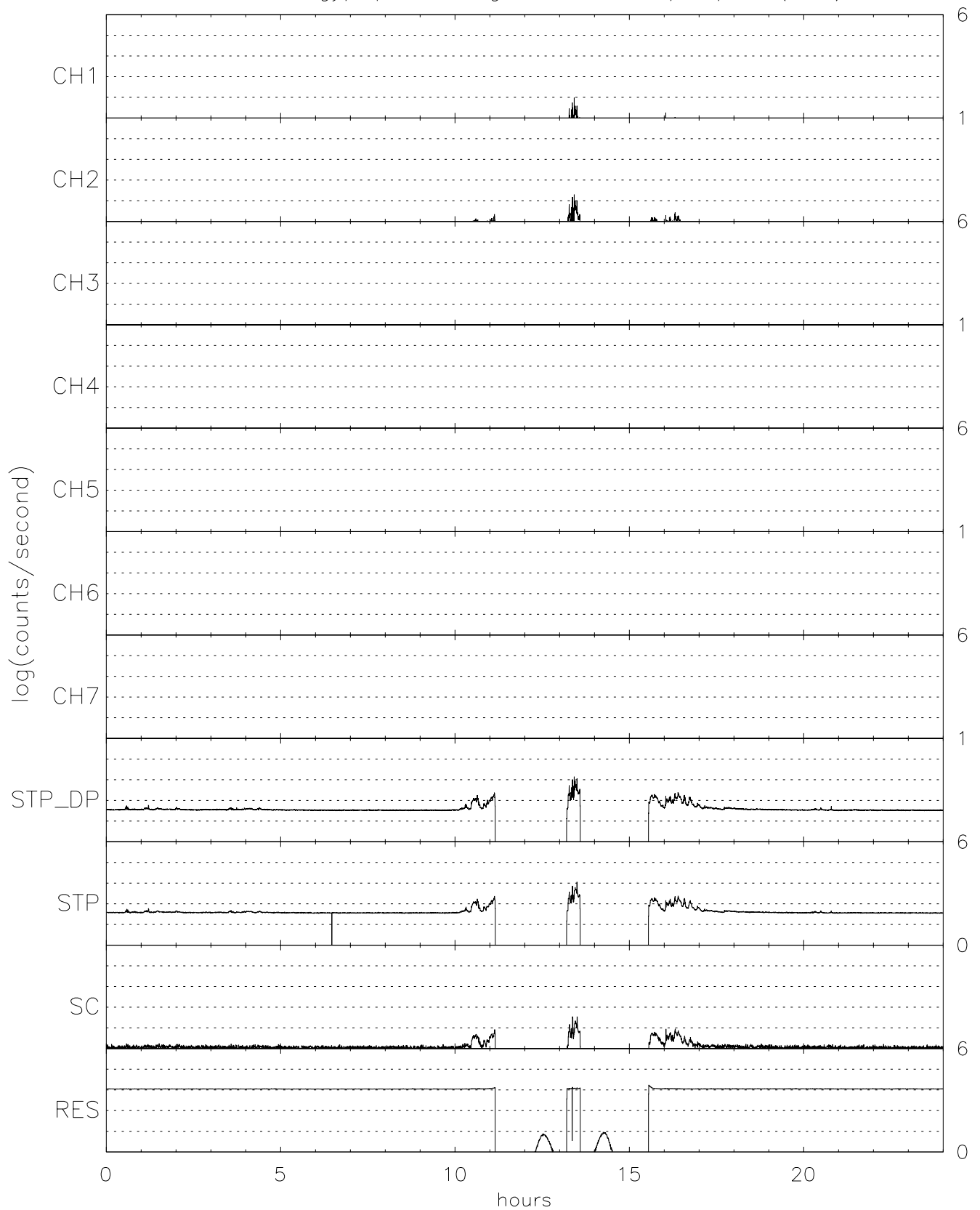
TIDE energy/spin averaged H+ for 02/25/97 (056)
