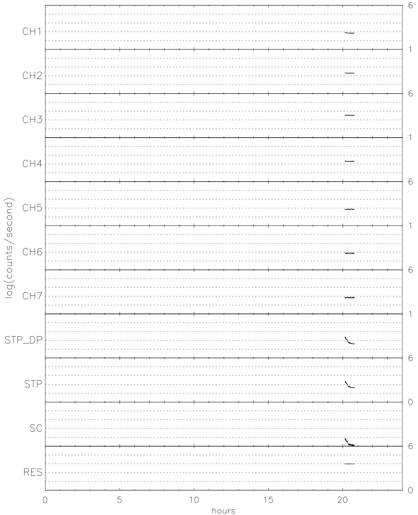
TIDE energy/spin averaged Singles for 02/19/97 (050)
