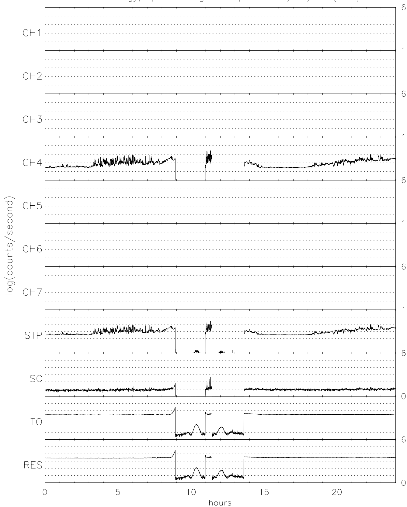
TIDE energy/spin averaged Stops for 01/15/97 (015)
