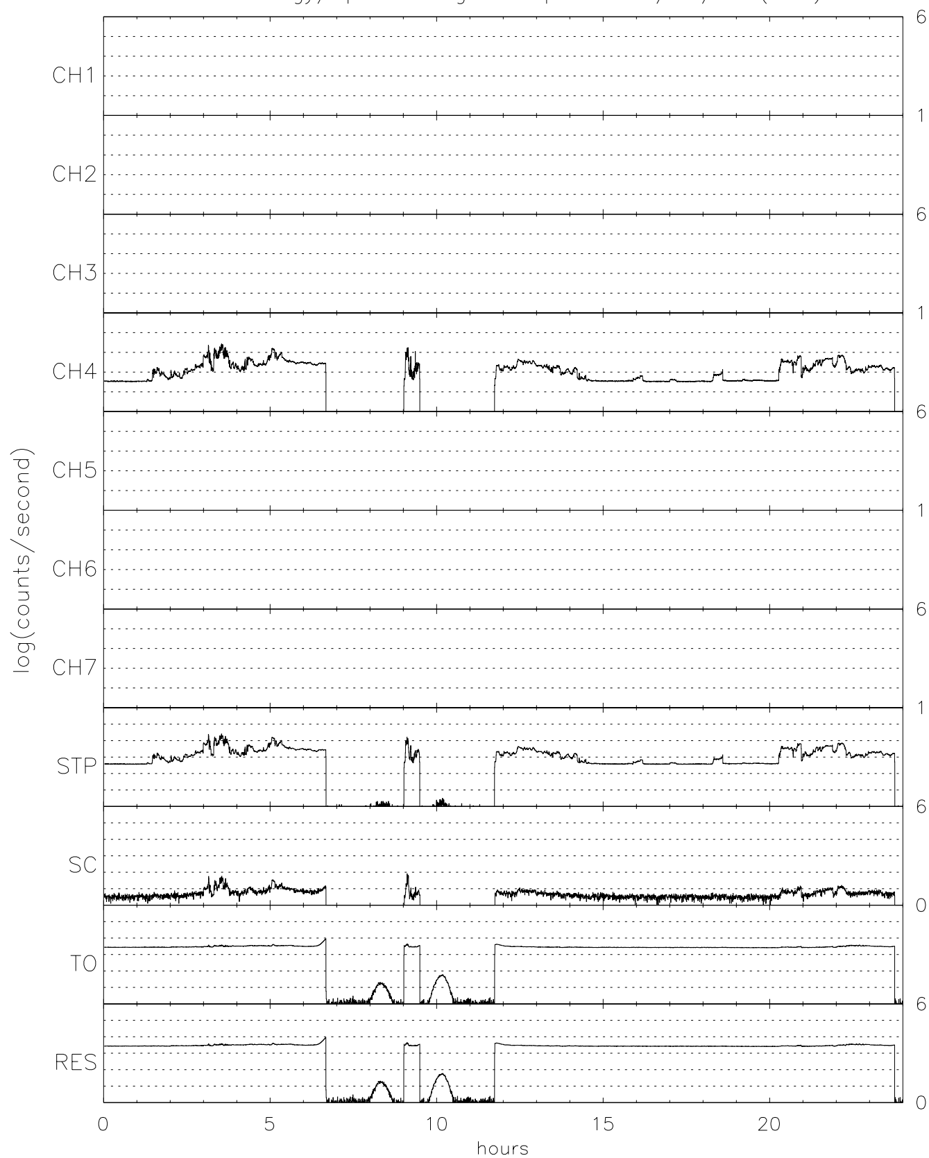
TIDE energy/spin averaged Stops for 12/27/96 (362)
